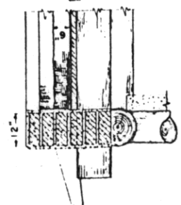
PORCH SECTION C-C ALTERNATE DESIGN SCALE 1/2" = 1'-0"
